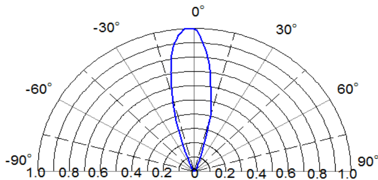
Figure4. Relative Luminosity VS. Radiation Angle
