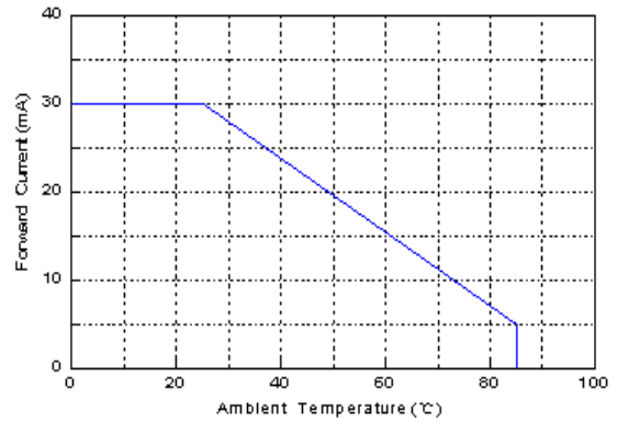
Figure2. Forward Current VS. Ambient Temperature;
