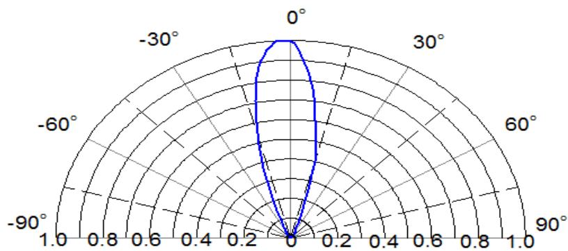
Figure4. Relative Luminosity VS. Radiation Angle
