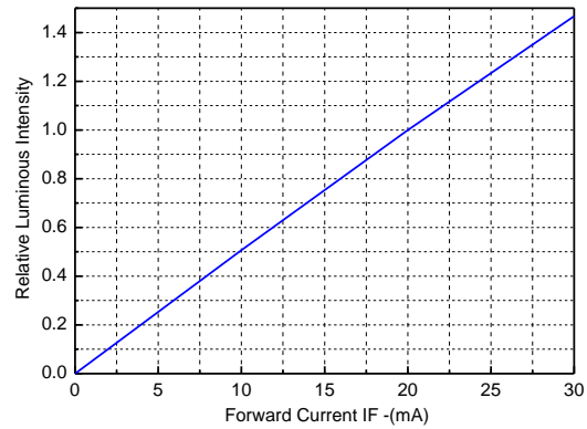
Figure4. Relative Luminous Intensity vs. Forward Current
