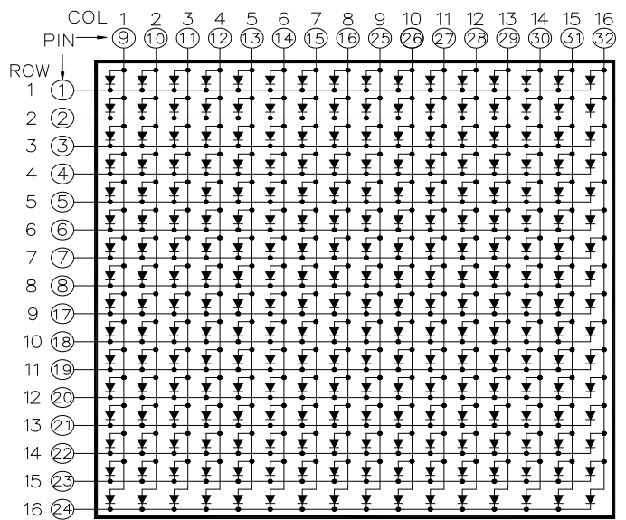
CSDM-16101 Common Column Anode
