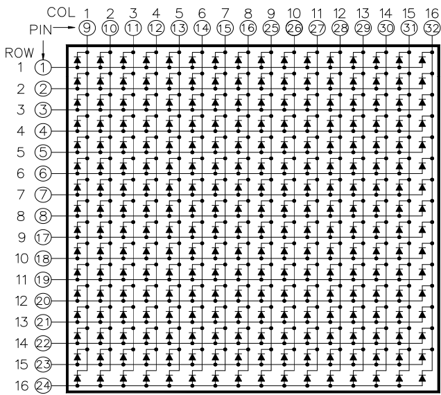
CSDM-16100 Common Column Cathode
