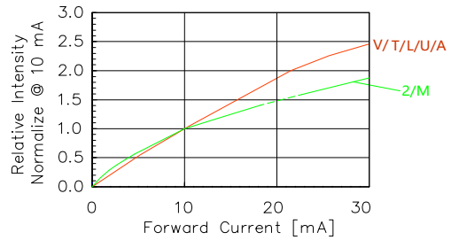
Fig 2. Relative Intensity vs. Forward Current
