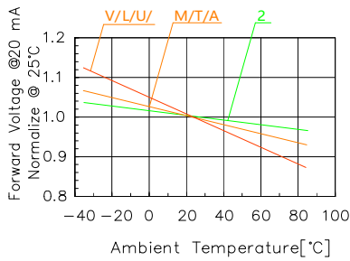
Fig 3. Forward Voltage vs. Temperature
