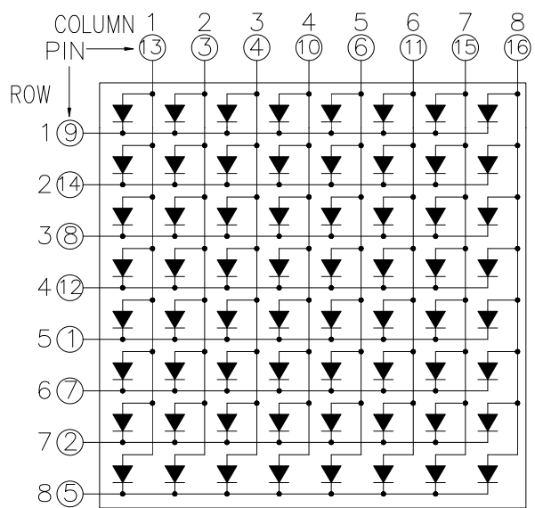
CSOM-88111 is Common Column Anode
