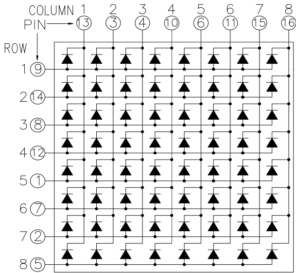
CSOM-88110 is Common Column Cathode
