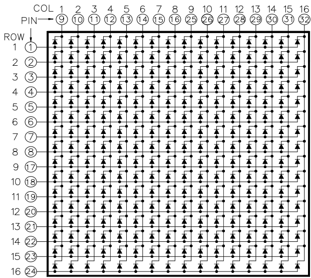
CSOM-16100 is Common Column Cathode
