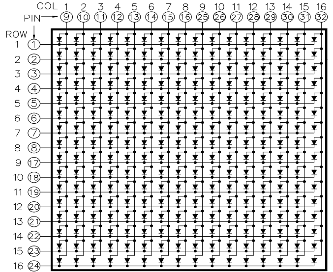
CSOM-16101 is Common Column Anode
