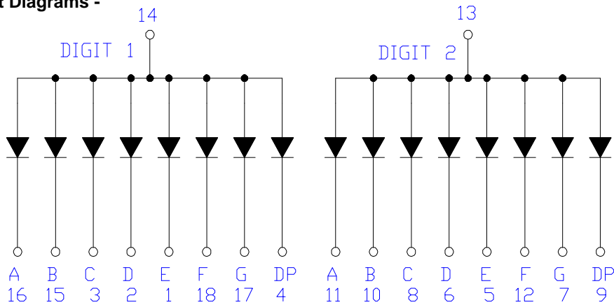
CSOD-56200 is Common Anode
