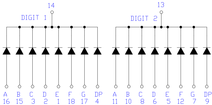
CSOD-56201 is Common Cathode
