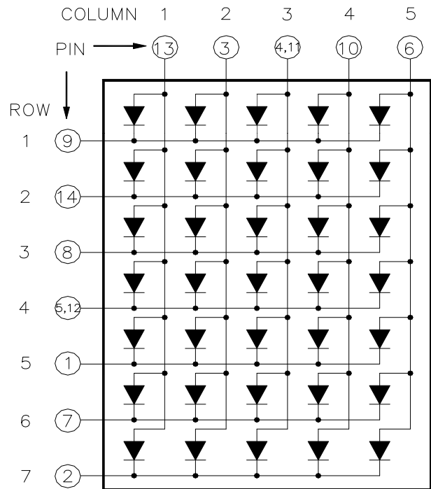
CSDM-57105 is Common Column Anode
