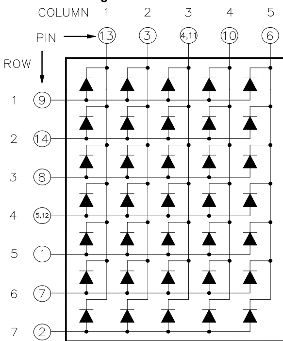
CSDM-57104 is Common Column Cathode
