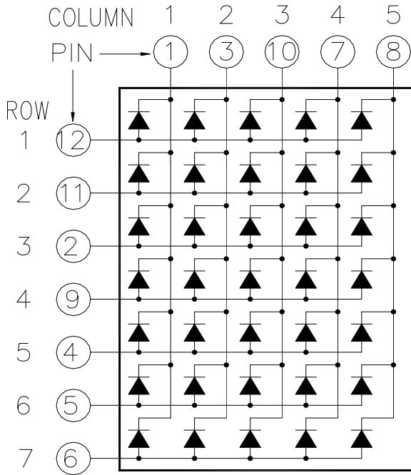
CSOM-57004 is Common Column Cathode
