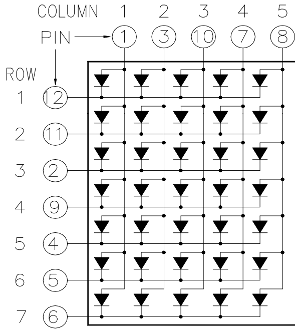
CSOM-57005 is Common Column Anode
