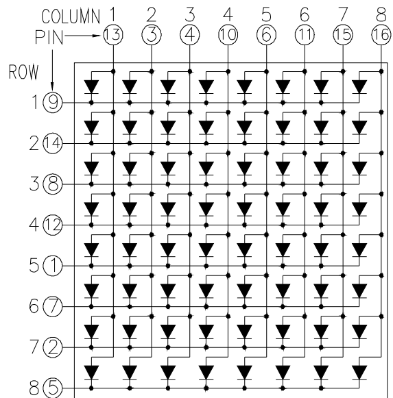
CSOM-88107 is Common Column Anode
