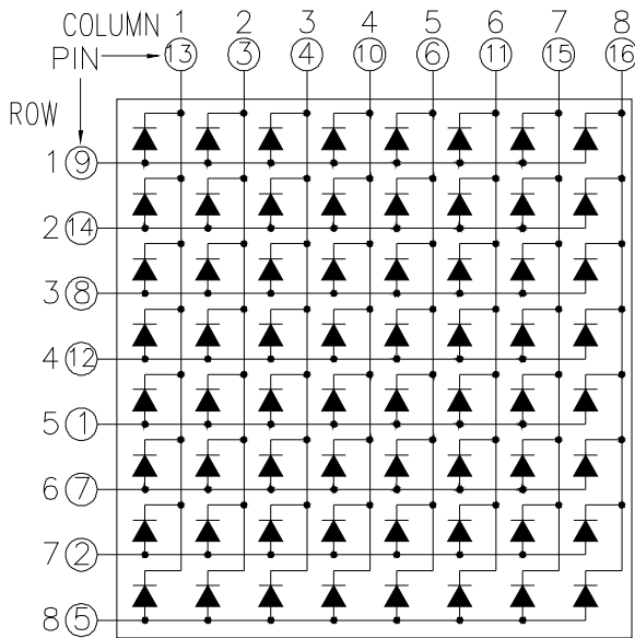
CSOM-88106 is Common Column Cathode
