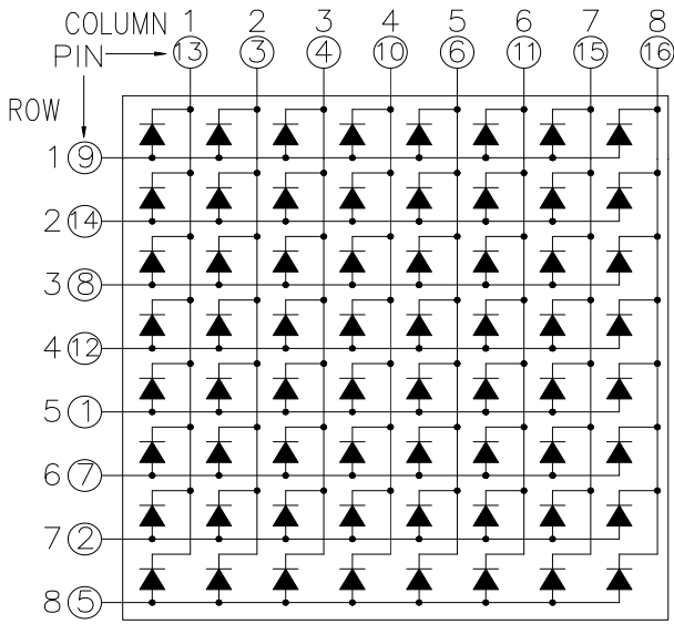
CSOM-88114 is Common Column Cathode
