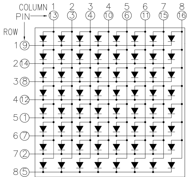
CSOM-88115 is Common Column Anode
