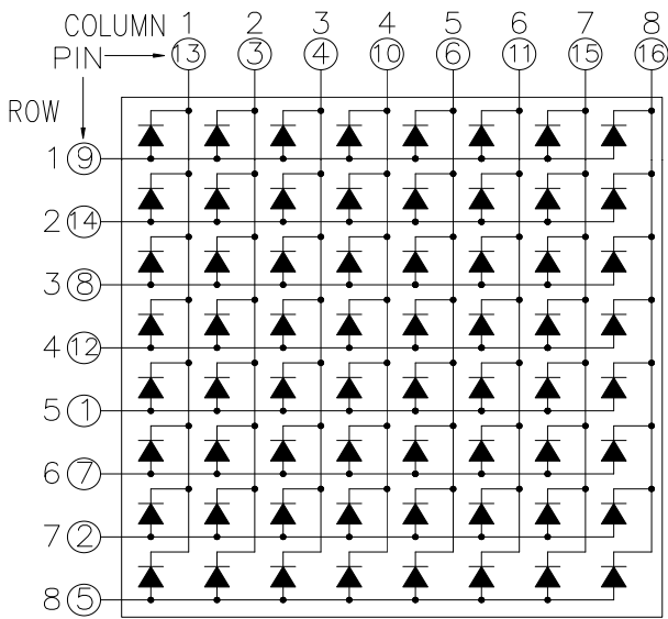
CSOM-88204 is Common Column Cathode
