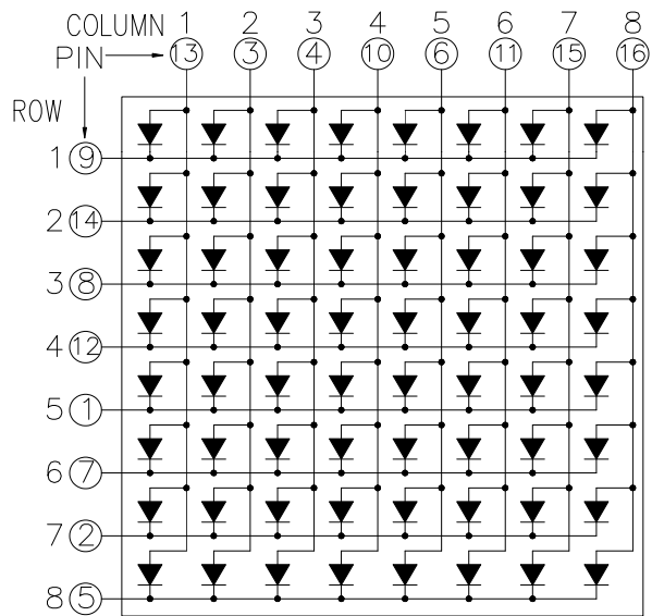
CSOM-88205 is Common Column Anode
